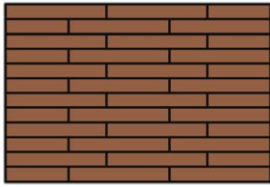
Less than 16m 2 : full loose lay installation – no expansion gap
